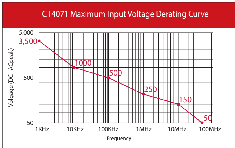
Figure 2 CT4071: Derating Curve
